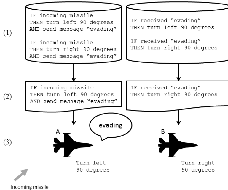
Figure 2. Example of DS+C in action. (1) Proactive and reactive coordination rules are added to the rule bases. The left rule base shows two example proactive rules, the right rule base shows to example reactive rules. Variations on the same rules are made to give the DS algorithm more options to explore. (2) The DS algorithm selects rules from the rule bases to form scripts (in this case, one rule per script). (3) Agent A’s rule is activated by an incoming missile. A turns, and sends a message “evading” to B. This activates B’s rule, causing B to turn.
