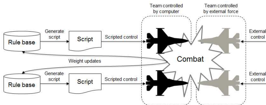
Figure 1. Dynamic scripting in the context of two learning agents in an air combat simulation.
