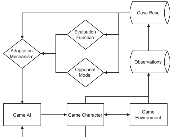
Figure 1: Rapidly adaptive game AI (see text for details).
